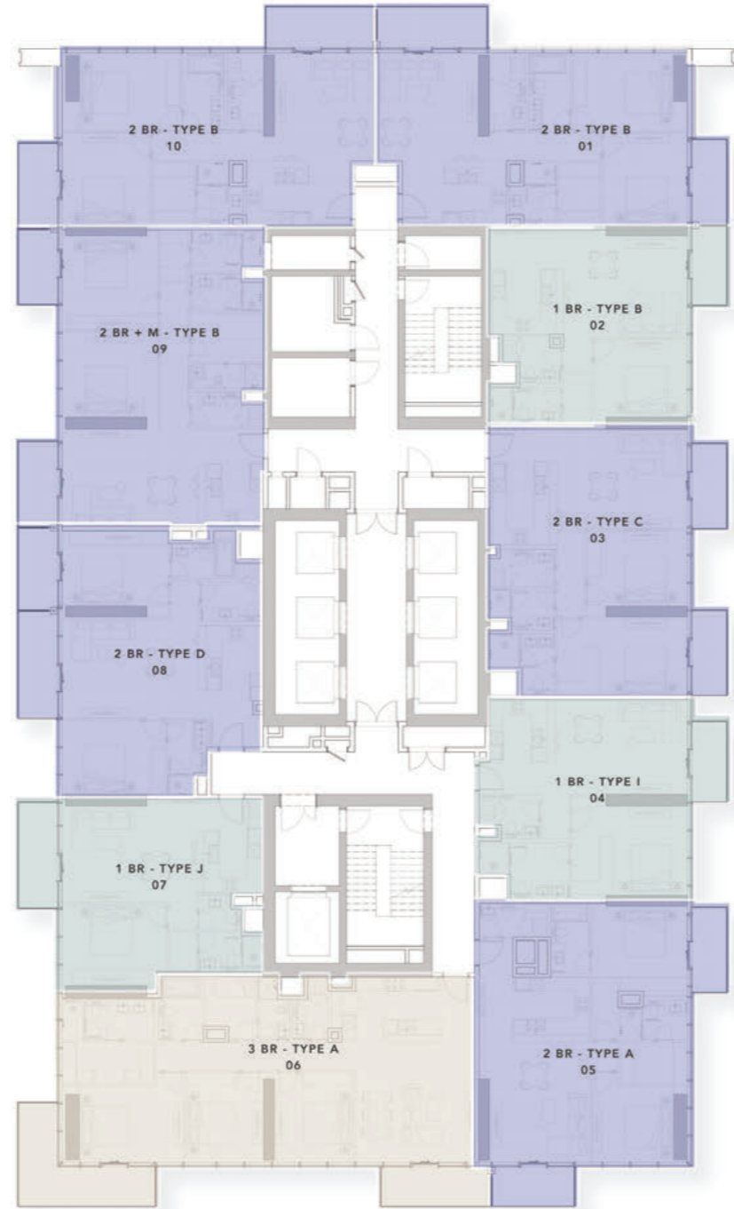
LEVEL 18-19 & 23-30 TYPICAL FLOOR PLAN
