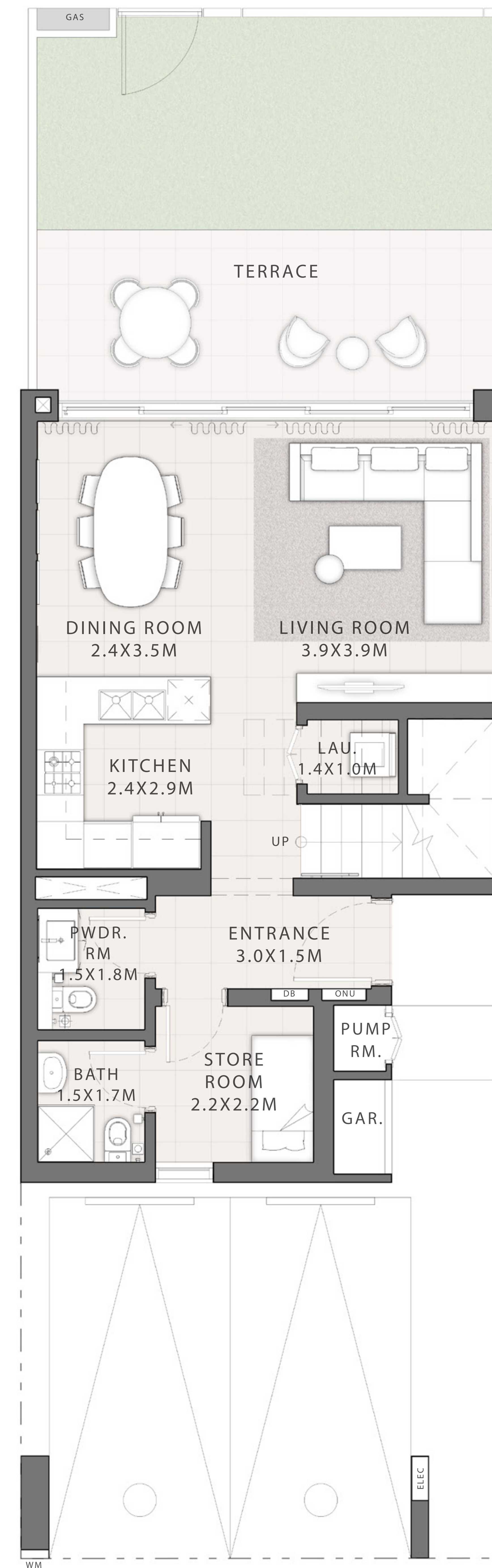
GROUND FLOOR
