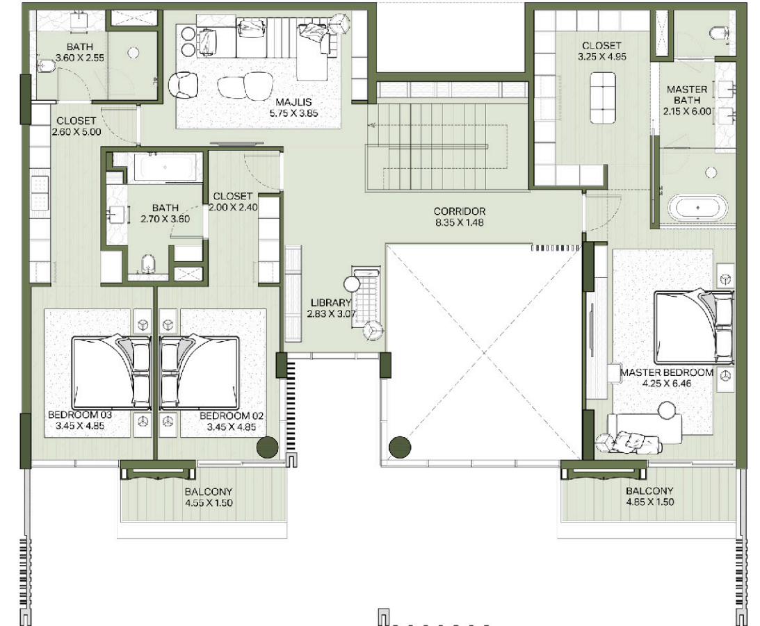
UPPER LEVEL
