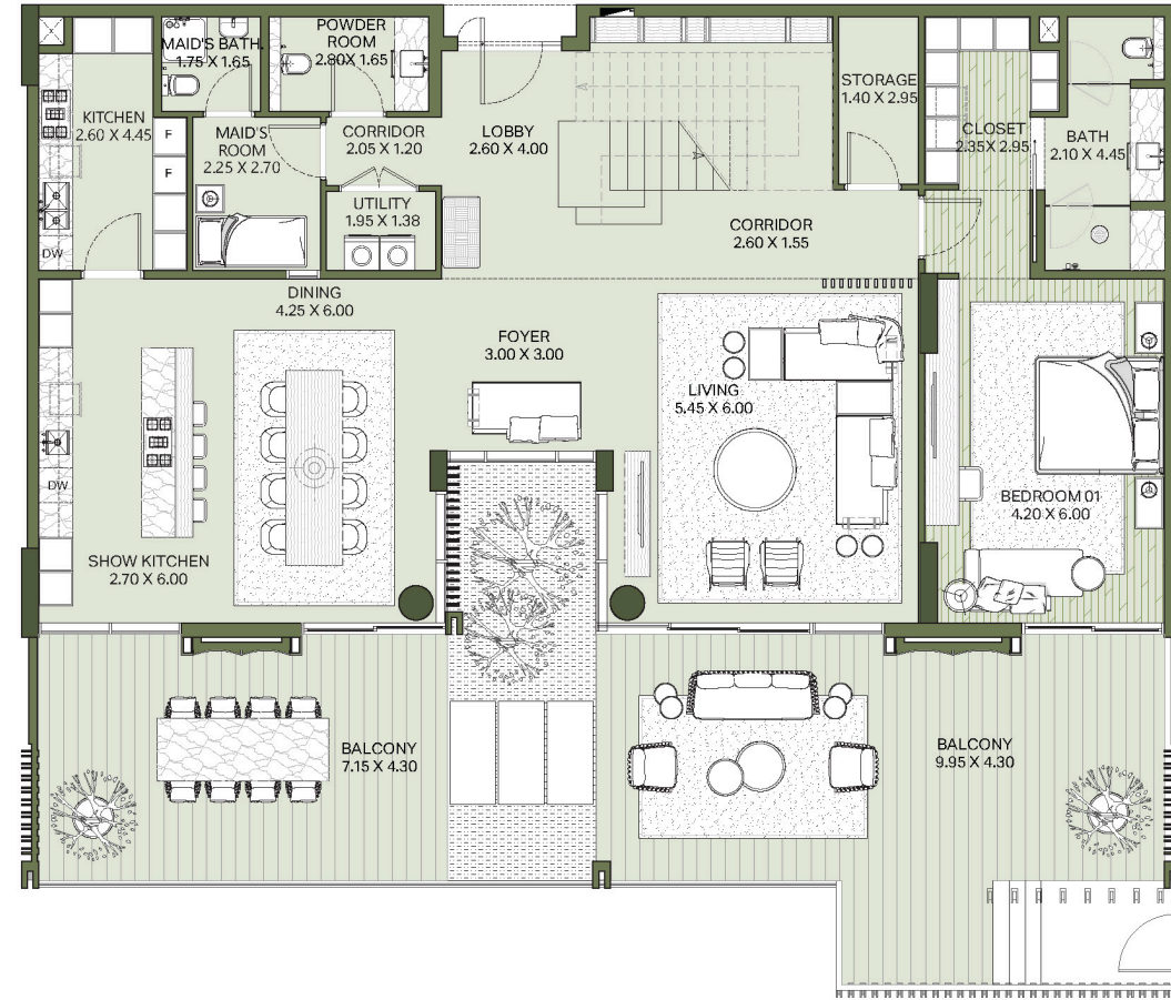
LOWER LEVEL
